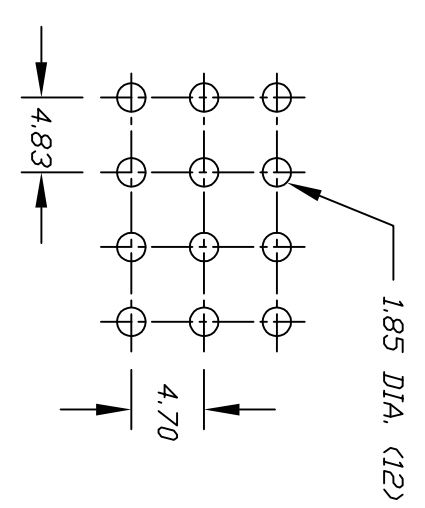
P.C.B MOUNTING HOLES
