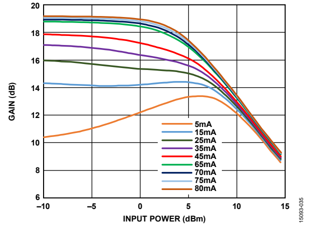
Figure 35. Gain vs. Input Power for Various Supply Currents ( I_{DQ} ) at 5 GHz, V_{DD} = 5 V
