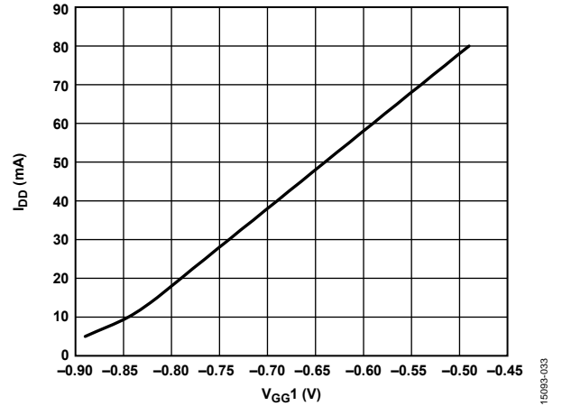
Figure 33. Supply Current with RF Applied ( I_{DD} ) vs. V_{GG1} , V_{DD} = 5 V, Representative of a Typical Device
