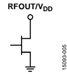
Figure 5. RFOUT/V DD Interface Schematic
