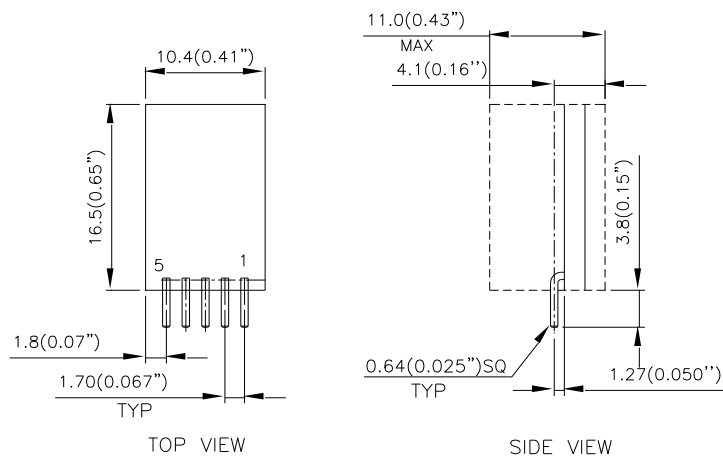
PIN ASSIGNMENT
