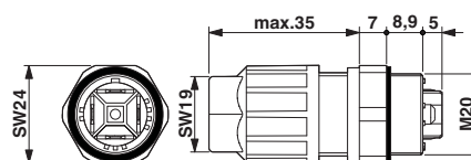
Dimensional drawing
